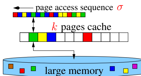
Figure 13.1: Paging in a virtual memory system
