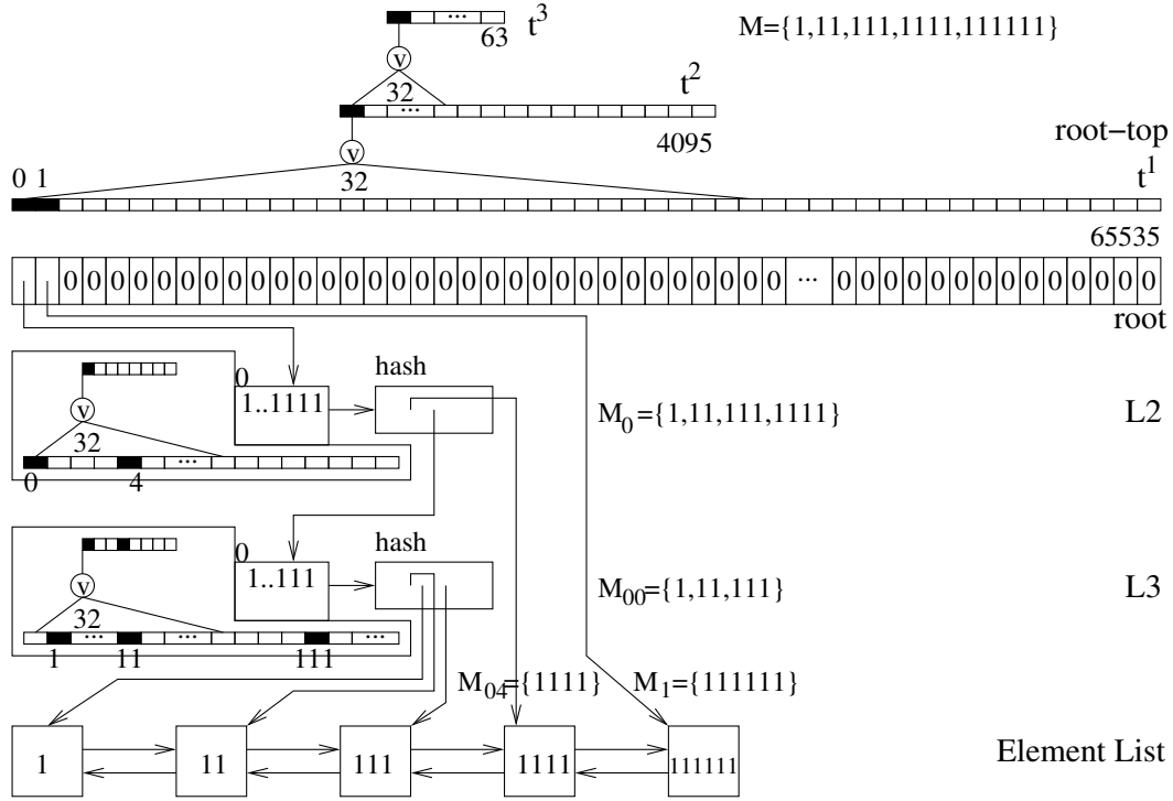
Figure 1: The Stree-data structure for M = \{1, 11, 111, 1111, 11111\} (decimal).
