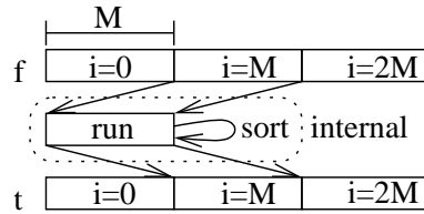
Figure 7.3: Run formation
