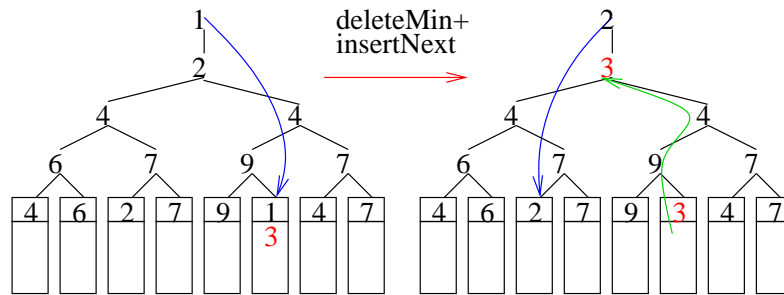
Figure 7.7: A tournament tree
