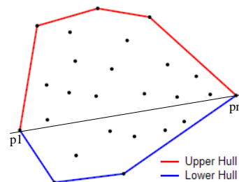
Figure 10.4: Upper/Lower Hull
