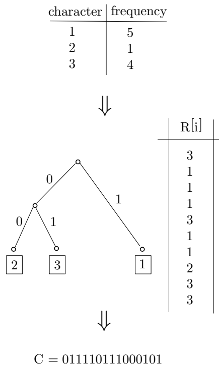
Figure 9.16: Huffman Encoding.
